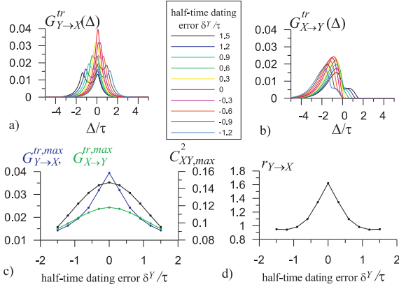
Fig. 1: (Colour online) Causality measures depending on dating error \delta^Y for the system (2) at h/\tau = 0.2 and \sigma_{\Xi}^2 = \sigma_{\Psi}^2 = 0 , k/\alpha is such that C_{X_0 Y_0, 0}^2 = 0.1 , l_X = l_{XY} = l_Y = l_{YX} = 1 : ((a), (b)) truncated WG causalities vs. time lag for different dating errors; (c) maximal truncated WG causalities (blue and green) and maximum CCF value (black) and (d) causality ratio vs. \delta^Y .
