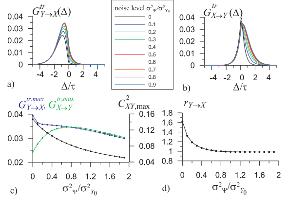
Fig. 2: (Colour online) Causality measures depending on observational noise level \sigma_{\Psi}^2 for the system (2) at h/\tau = 0.2 , \sigma_{\Xi}^2 = 0 , \delta^Y = 0 , C_{X_0 Y_0, 0}^2 = 0.1 , and l_X = l_{XY} = l_Y = l_{YX} = 1 : ((a), (b)) truncated WG causalities vs. time lag for different noise levels; (c) maximal truncated WG causalities (blue and green) and maximal CCF value (black) and (d) causality ratio vs. \sigma_{\Psi}^2/\sigma_{Y_0}^2 .
